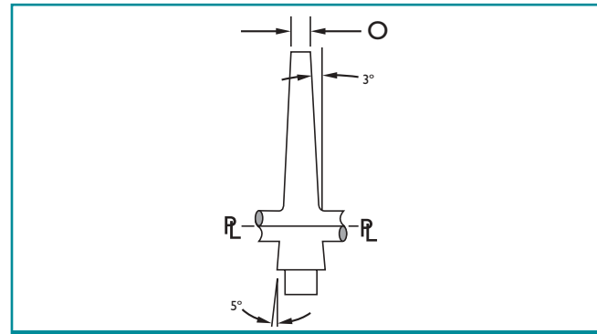
Figure 9. Conventional sprue.
