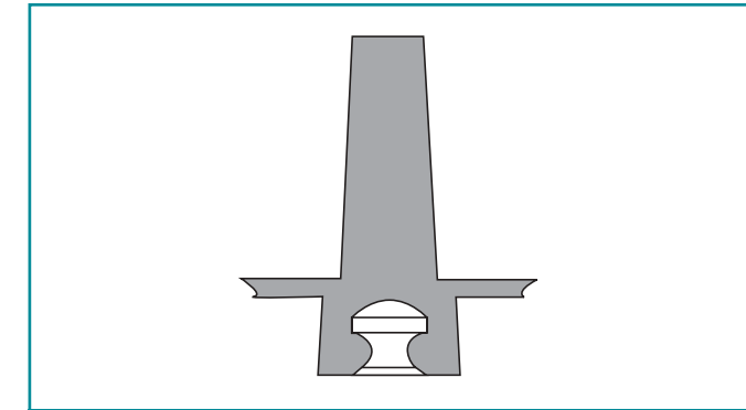
Figure 11. Buttonhead sprue puller for automated removal.
