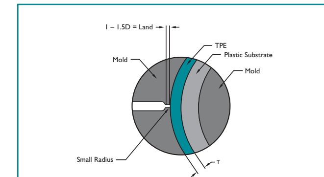
Figure 12. Tab/edge gate.
