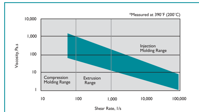
Figure 15. The effect of shear rate on the viscosity of GLS styrenic TPE compounds.
