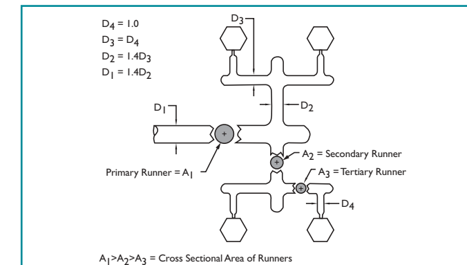
Figure 7. Runner design guidelines.
