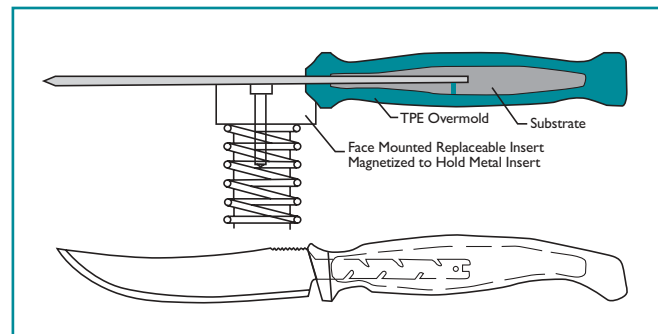
Figure 1. Spring-loaded insert for metal tolerances.
